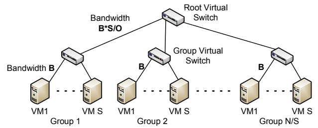
Figure 3: Virtual Oversubscribed Cluster abstraction.
