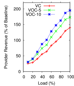
Figure 14: Provider revenue with virtual network abstractions. Mean Bandwidth = 500Mbps.
